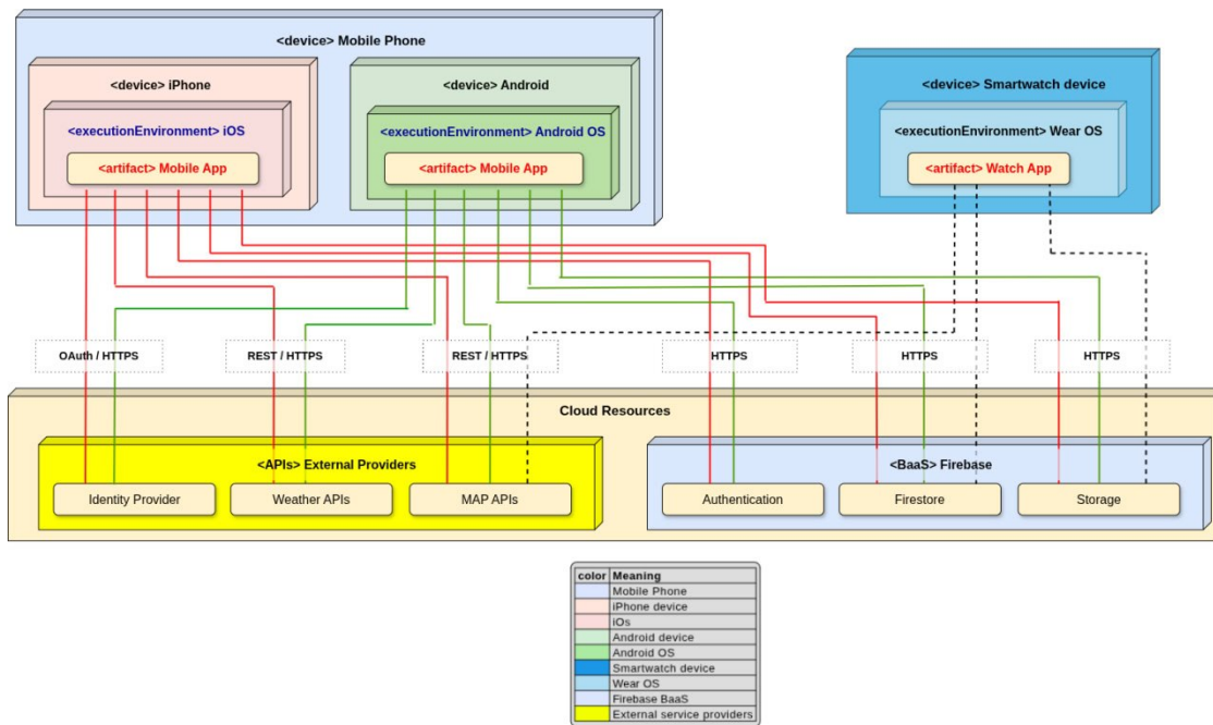
Figure 2.5: Deploy Diagram
